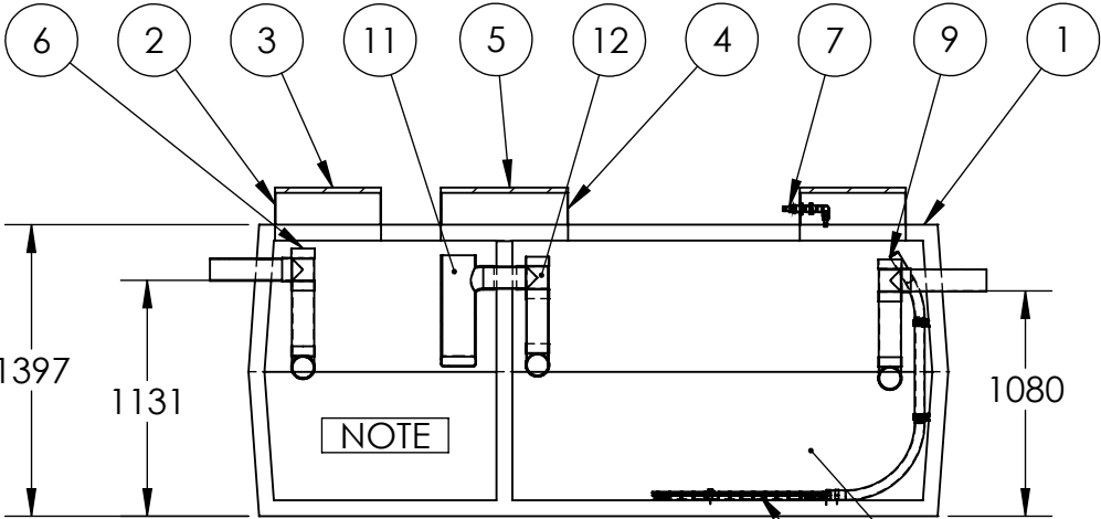
SECTION VIEW A-A BST-1700-RO
