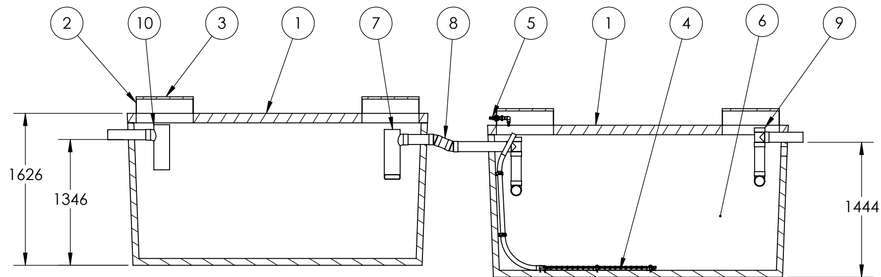
SECTION VIEW A-A BTT-3400-RO
